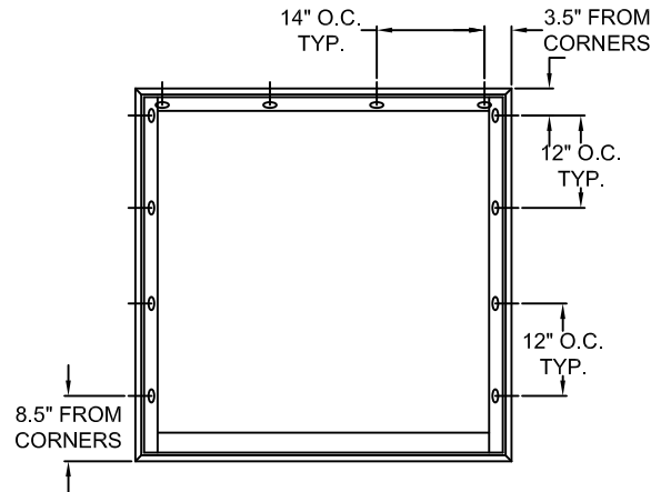
TYPICAL ELEVATION WITH FASTENER SPACING
