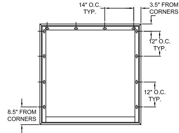
TYPICAL ELEVATION WITH FASTENER SPACING
